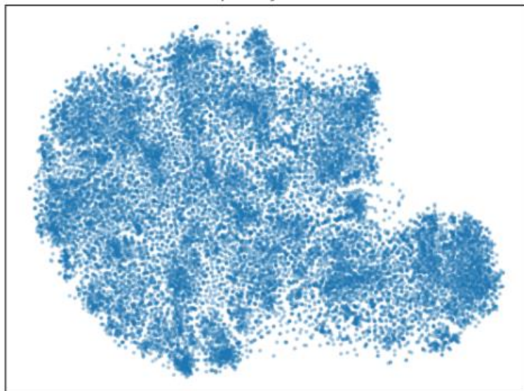
Perplexity = 150
