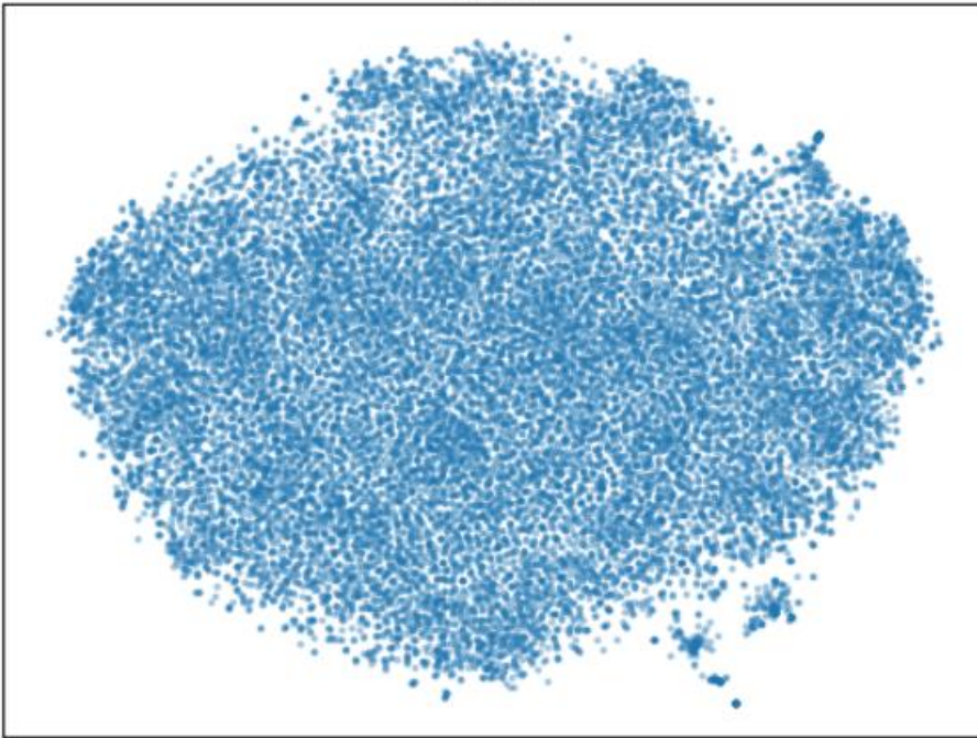
spacy
